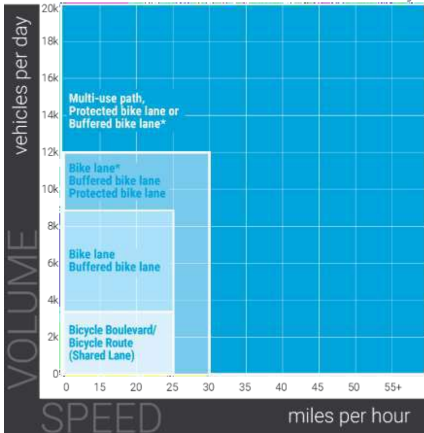
Figure 4.4. Bicycle Facility Selection Chart
